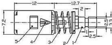
Outline Drawing
