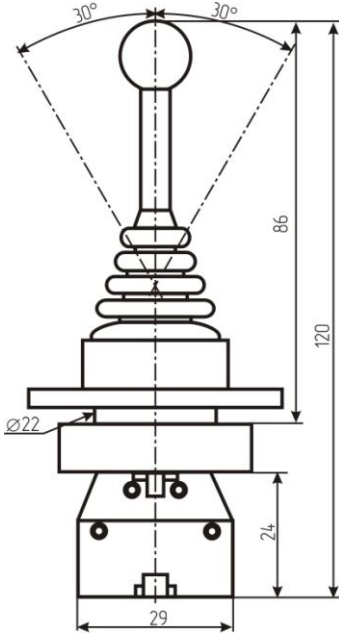
Outline Drawing
